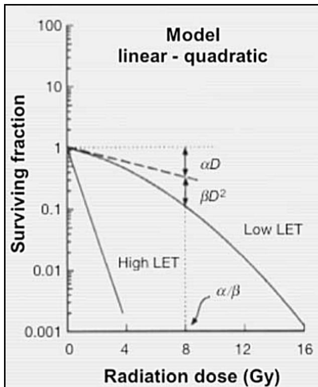
Figure 2: Linear Quadratic Model of Cell Survival
