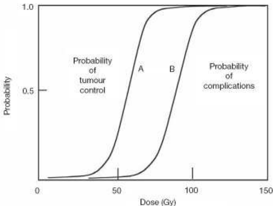
Figure 1: The principle of therapeutic ratio. Curve A represents the TCP, curve B the probability of complications. The total clinical dose is usually delivered in 2 Gy fractions.
