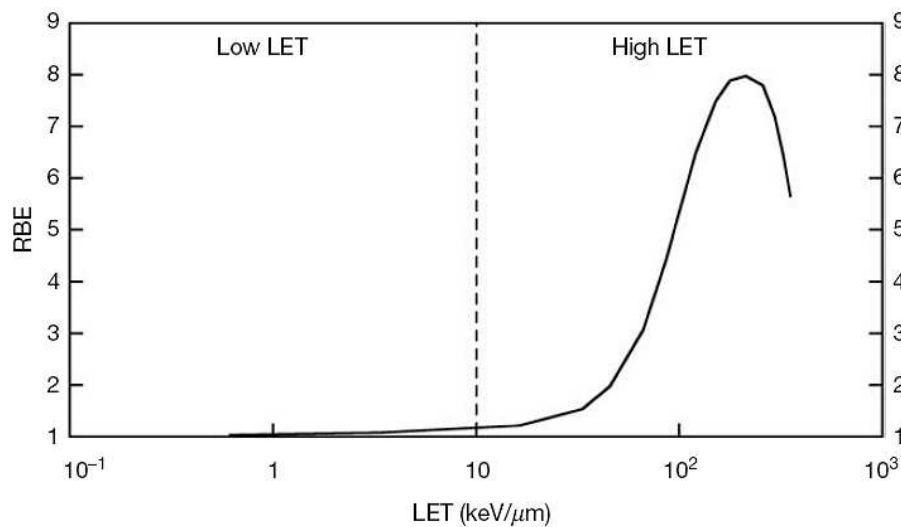
Figure 3: RBE v LET
