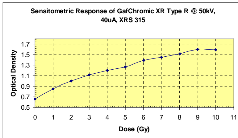
Figure 1: Sensitometric Response of GC-XRR film @ 50kV, 40uA.
